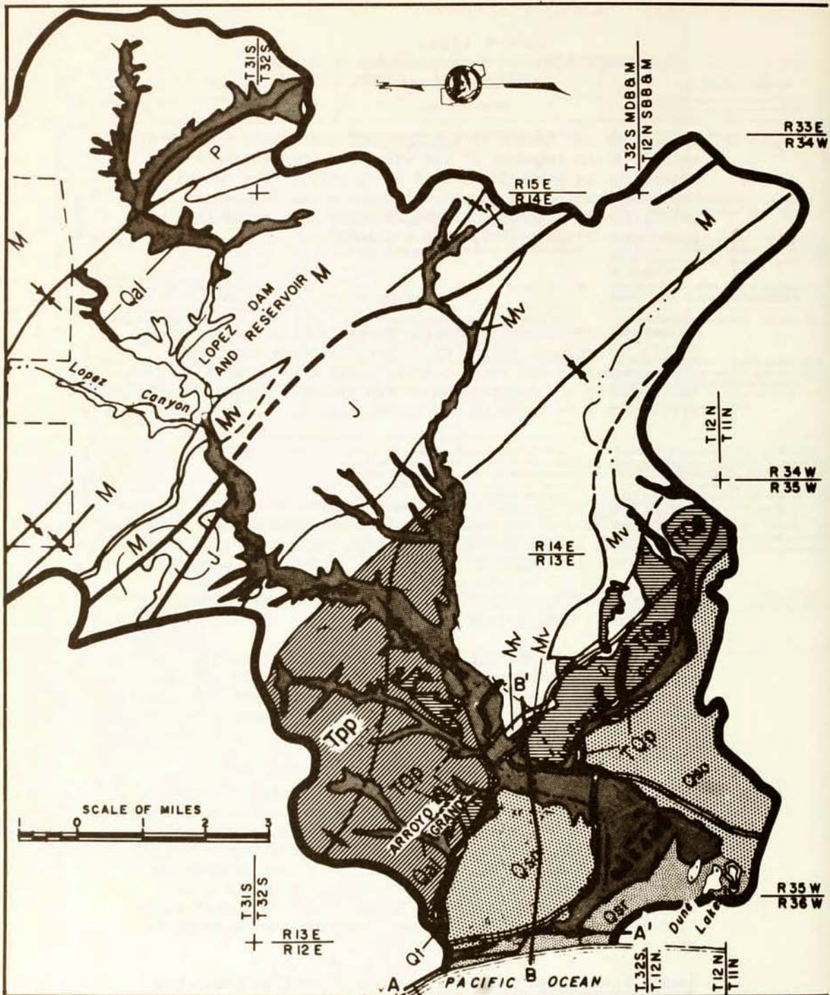
Figure 4 - AREAL GEOLOGY
